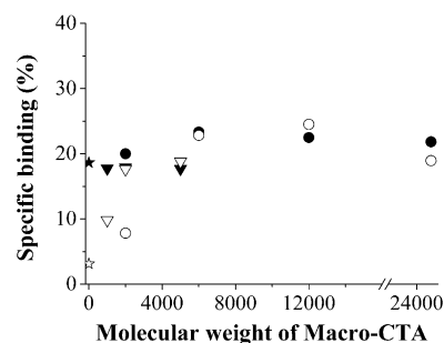
Figure 4. Specific template bindings on the ungrafted MIP microspheres (i.e., M_n of the Macro-CTA=0; star), the MIP microspheres grafted with PNIPAAm brushes ( M_n=1800 , 5900, 11 900, and 24 800; circle), and those grafted with PEG brushes ( M_n=1000 , 2000, and 5000; triangle) in a 2,4-D solution (0.08 mM) in methanol/water (4:1 v/v; filled symbols) and in pure water (open symbols) at 25 °C, respectively (polymer concentration: 16 mg mL -1 ).
